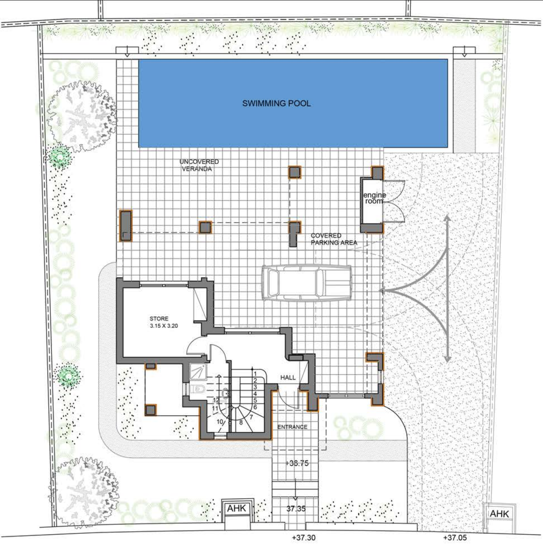
FIRST LEVEL PLAN
